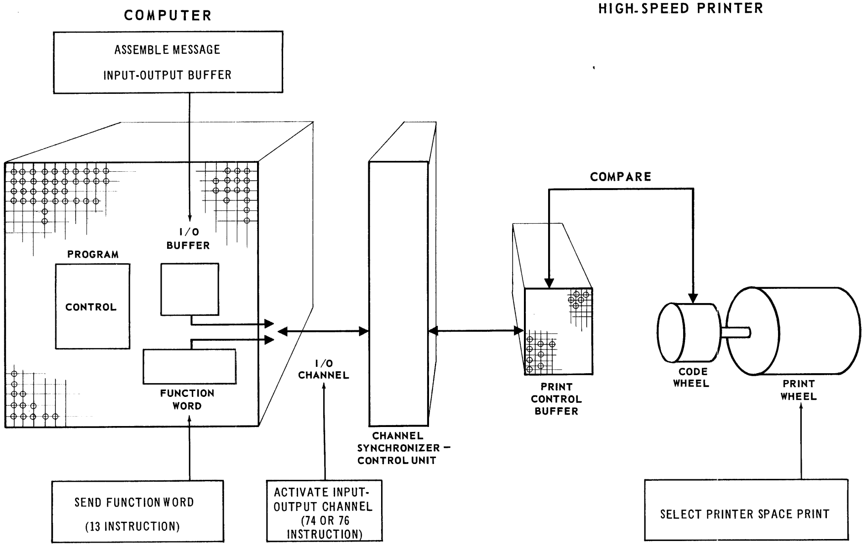
Figure 4-2. UNIVAC 490 Computer and the High-Speed Printer
